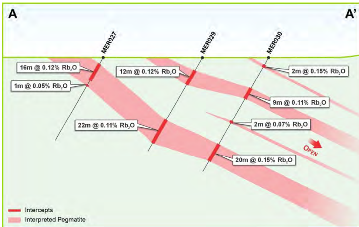
Figure 3: Section A-A' 6757870mN
